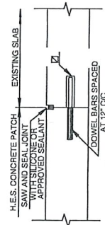
DETAIL OF TRANSVERSE JOINT (DOWEL BAR WITH CAP)
