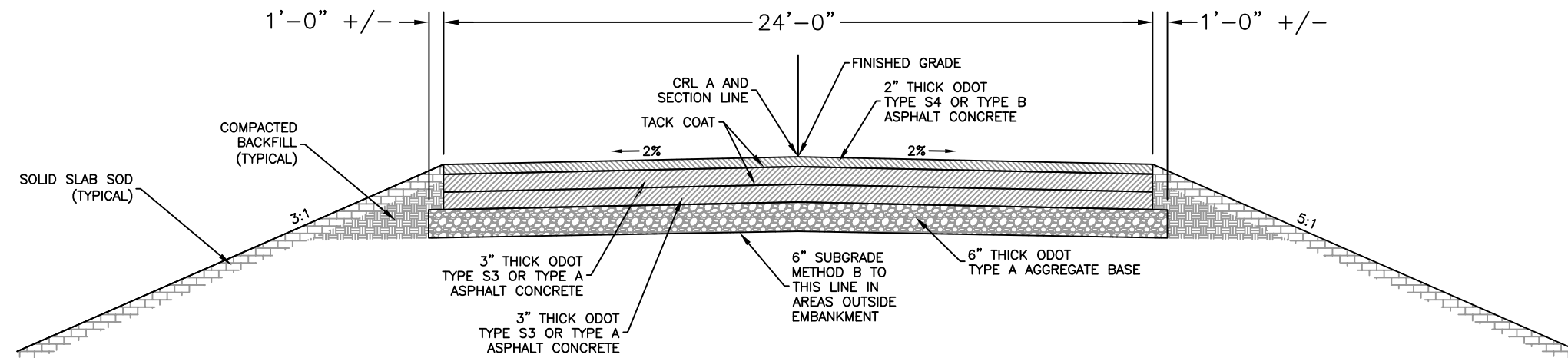
PAVEMENT REPAIR TYPICAL SECTION 9+40 TO 10+60 ASPHALT CONCRETE OPTION (NOT TO SCALE)
