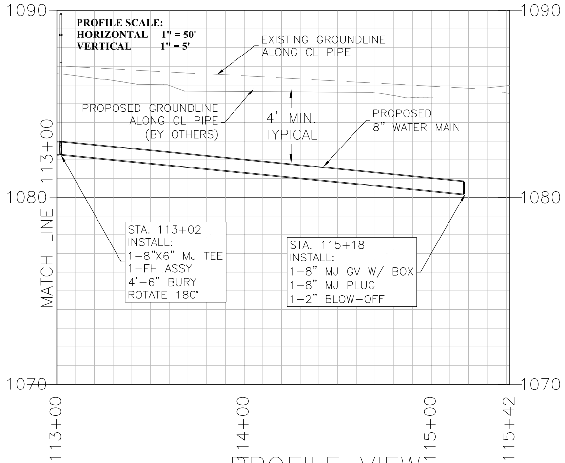
PROFILE VIEW
