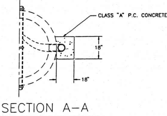
PIPE INSTALLATION DETAIL
