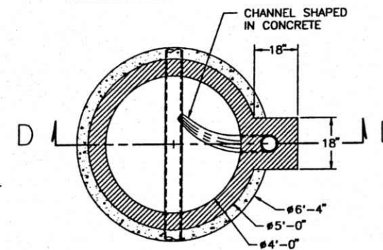
SECTION E-E
