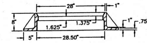
SECTION G-G
