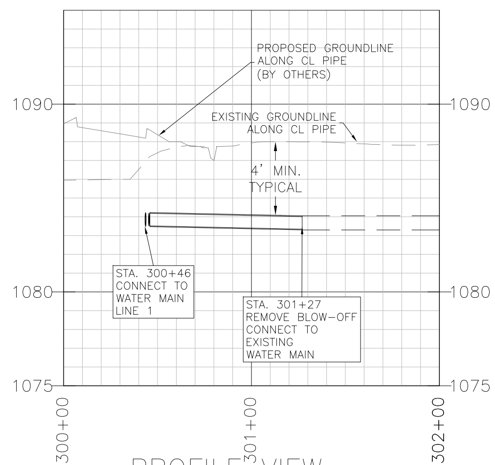
PROFILE VIEW
