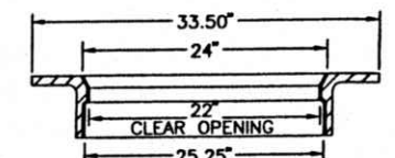
SECTION H-H
