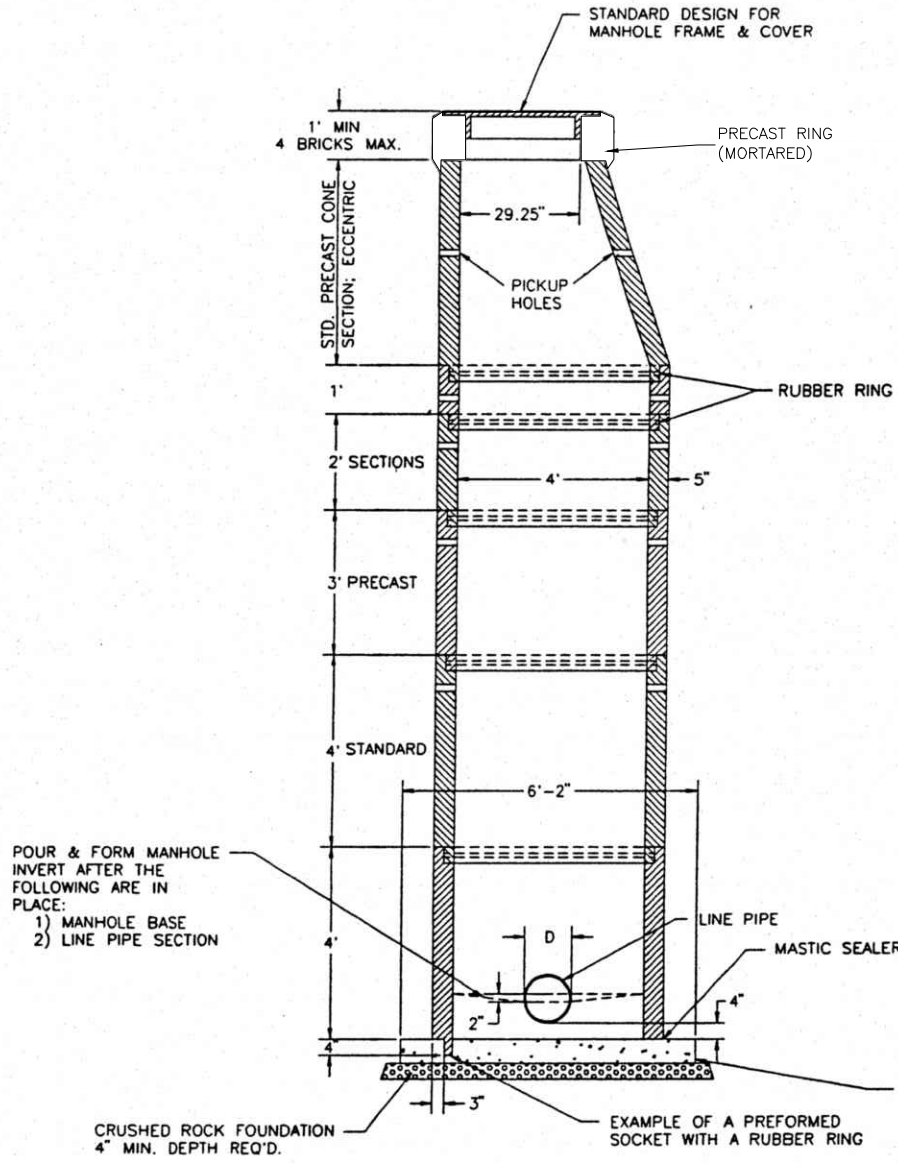
TYPICAL BASE DETAILS 4'-0" DIAMETER MANHOLE (Eccentric Cone)
