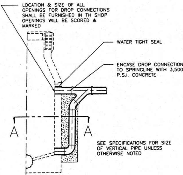
DROP MANHOLE CONNECTION
