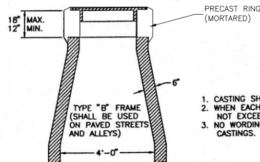
TYPICAL SECTION TO BE USED ON EXISTING AND FUTURE PAVING
